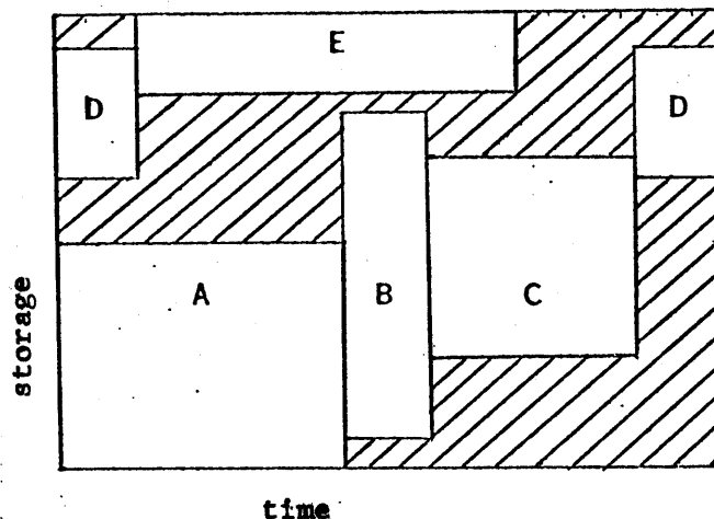
Figure IV-I, queue storage allocation.
