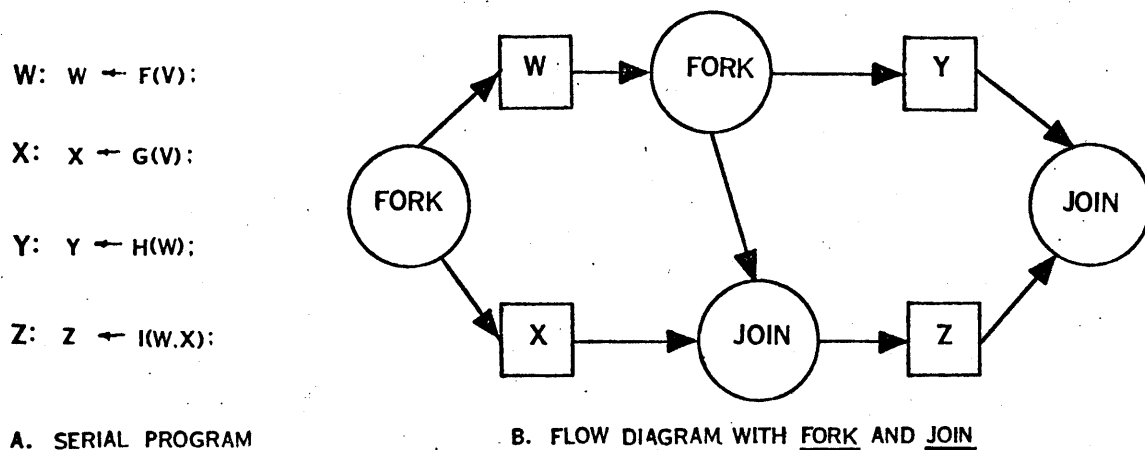
Figure II-A, nontransitivity of parallelism
