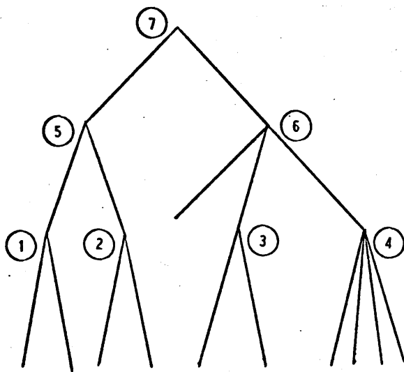
Figure VI-F, order of nonterminal nodes.
