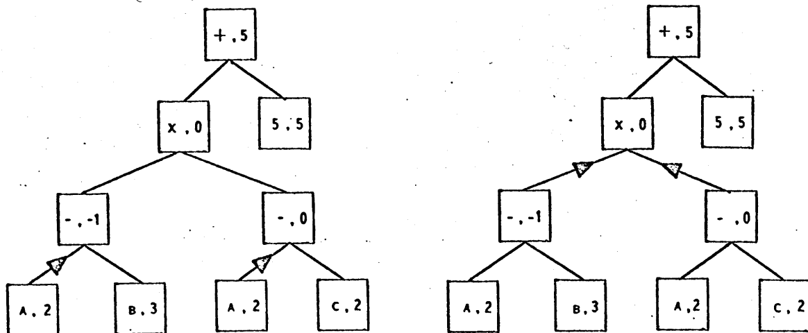
Figure VI-E, propagation by level.
