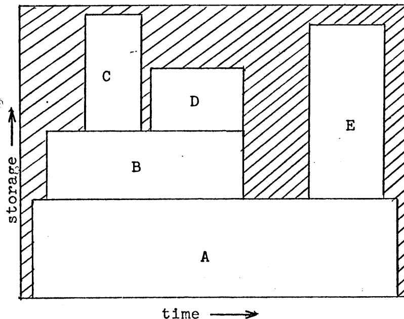
Figure IV-H, stack allocation.
