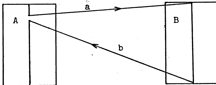
Figure IV-B, subroutine relation.
