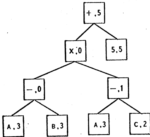
Figure VI-B, tree form.
