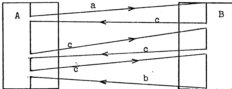
Figure IV-C, subordinate coroutine.
