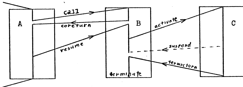
Figure IV-G, interface operations.
