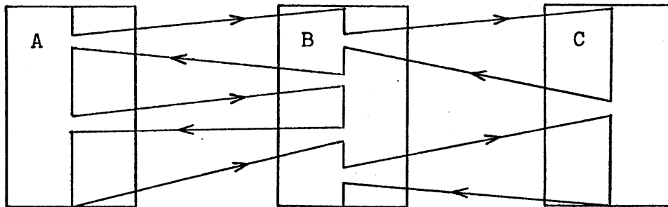
Figure IV-D, double coroutine without subordination between A and B or between A and C.
