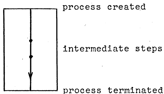
Figure IV-A, process diagram.
