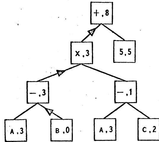
Figure VI-C, change propagation.
