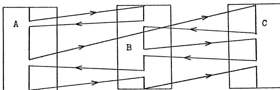
Figure IV-E, cyclic triple coroutine.
